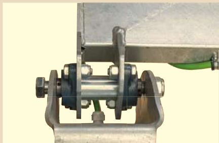
Massive Pendelachse
